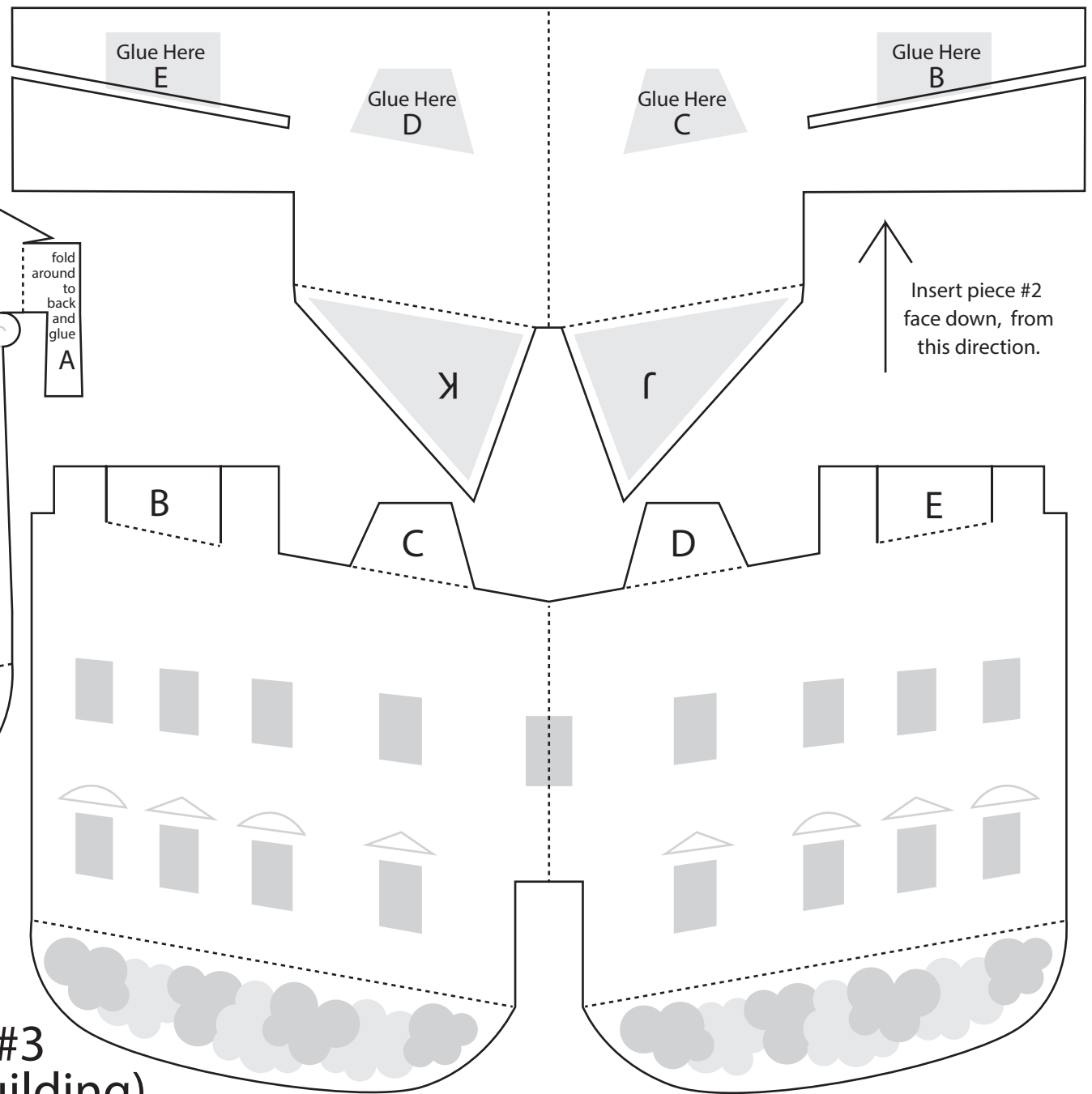
Piece #2 (roof)
